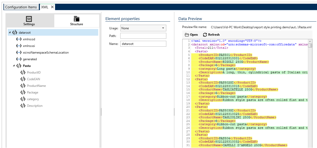
Configuring your XML data filter.
